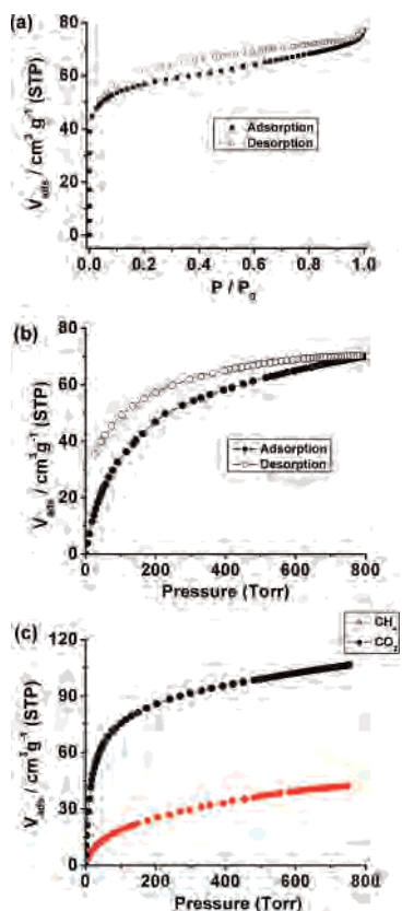
Figure 3. (a) Nitrogen sorption isotherm at 77 K. (b) Hydrogen adsorption–desorption isotherms at 77 K. (c) Carbon dioxide and methane adsorption isotherms at 195 K.
